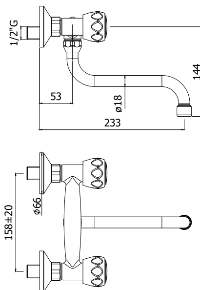
TECHNICAL DRAWING
