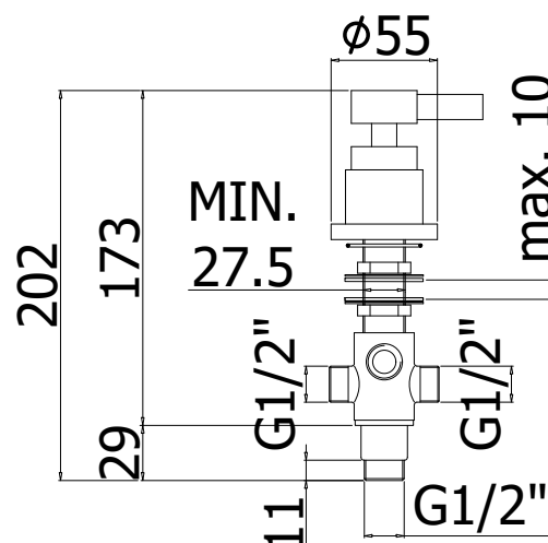
TECHNICAL DRAWING
