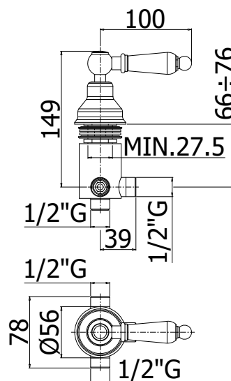
TECHNICAL DRAWING
