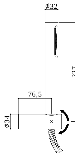
TECHNICAL DRAWING
