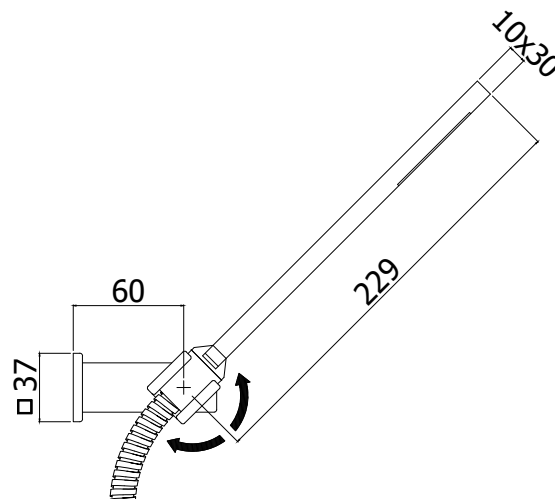
TECHNICAL DRAWING
