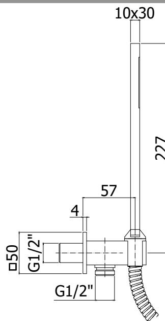
TECHNICAL DRAWING
