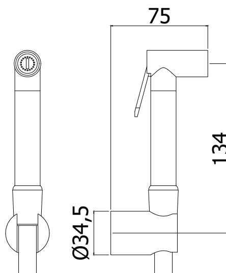
TECHNICAL DRAWING
