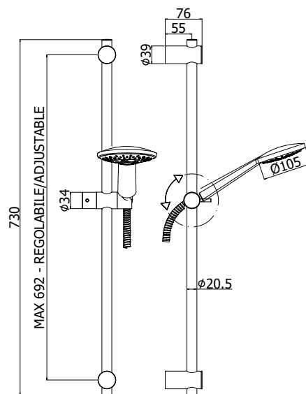
TECHNICAL DRAWING
