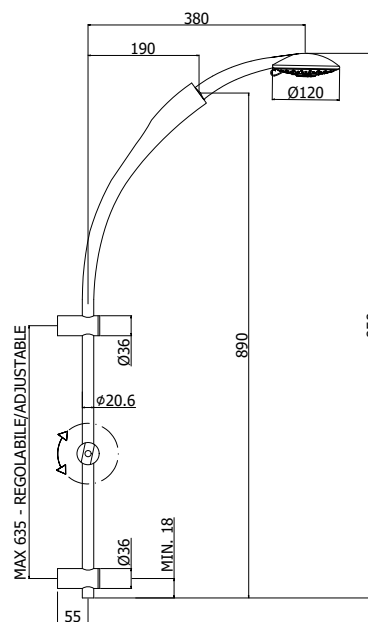
TECHNICAL DRAWING
