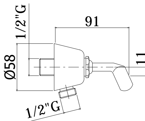
TECHNICAL DRAWING
